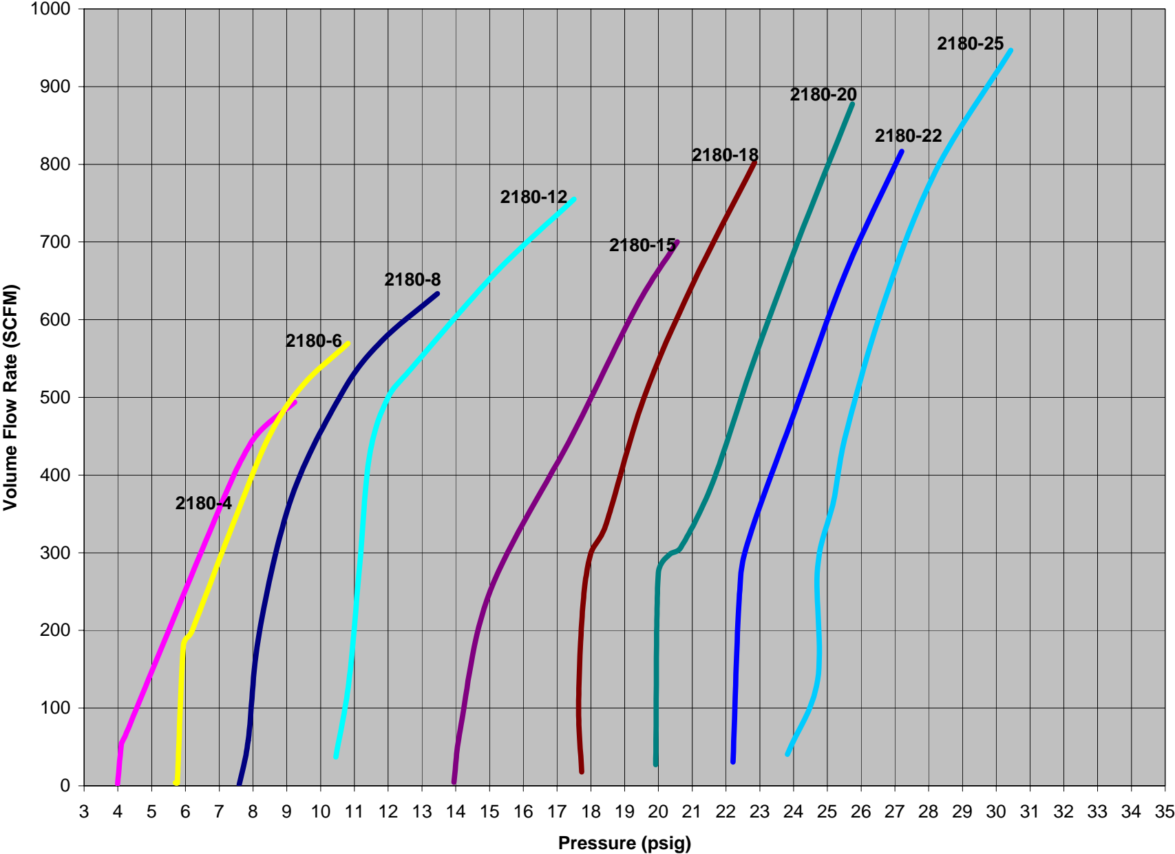
2180 Pressure Relief Valve - Flow Rate Vs Pressure
