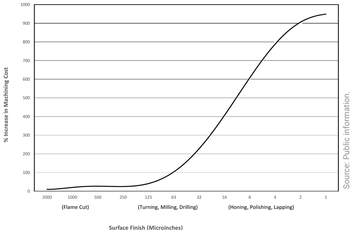
Fig.2 Increase in Machining Cost vs Surface Finish
